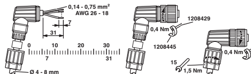
Functional drawing
